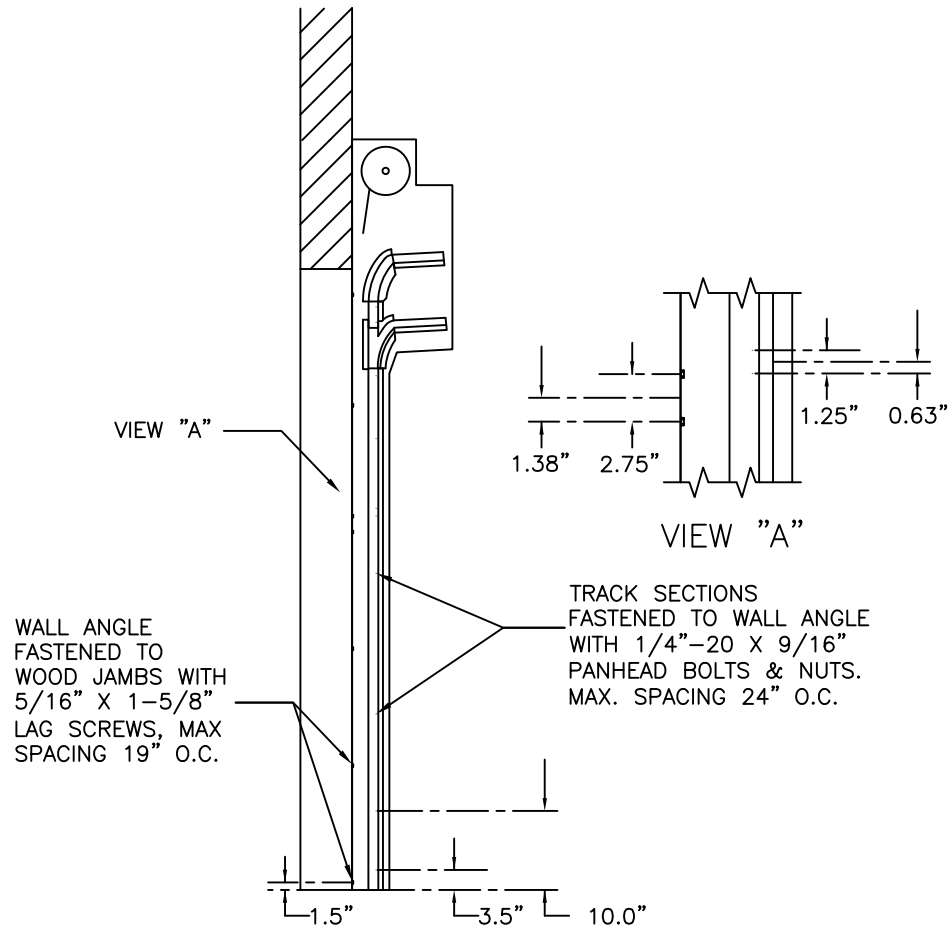
SIDE ELEVATION VERTI-STACK TRACK DETAILS
